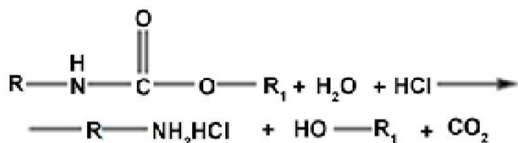
Figure 3. Acidolysis of PU foam
