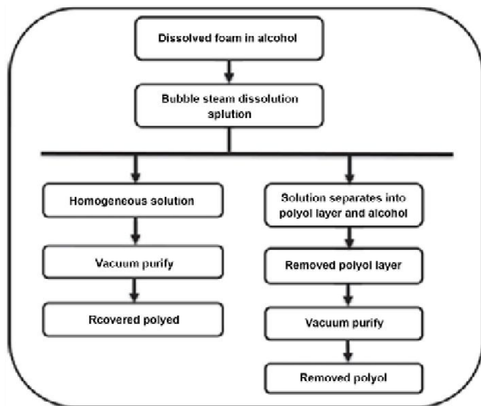
Figure 4. Hydroglycolysis recycling method.
