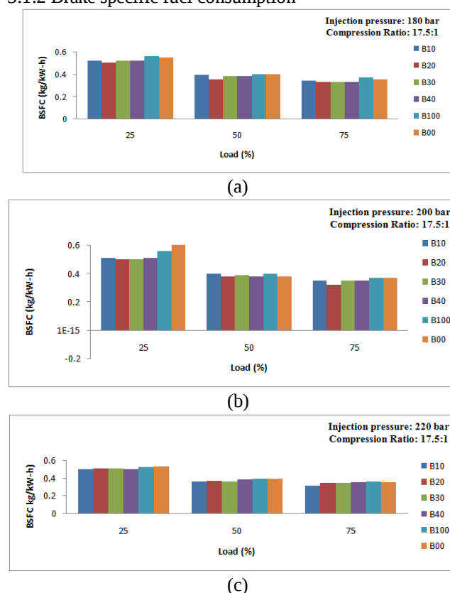
Fig.2 Variation of BSFC with respect to engine load (a,b,c)
