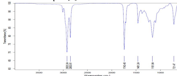
Fig.1. FTIR spectra of Argemone Mexican crude oil
