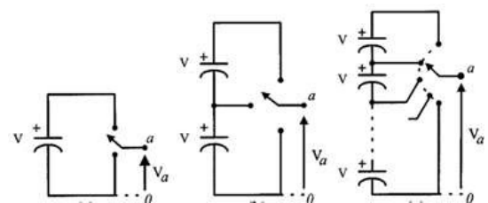
Fig.1. An Inverter with Two Levels, Three Levels And Multi Levels With One Phase
