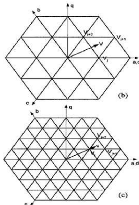
Figure.7: Space-Vector Diagram: (A) Two-Level, (B) Three-Level, and (C) Five-Level Inverter
