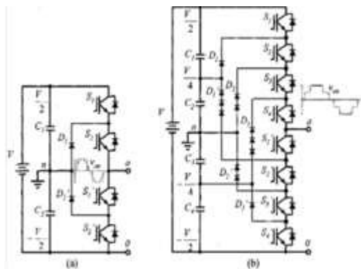
Fig.2: Diode-Clamped Multilevel (Three-Level & Five-Level) Inverter Circuit Topologies.
