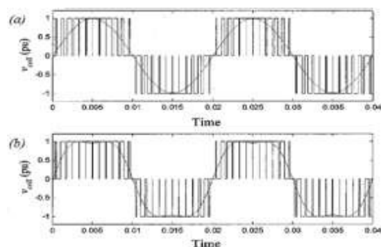
Figure.6: Inverter Cell Voltages. (A) Output Voltage and Reference with SPWM. (B) Output Voltage and Reference with Injection of Sinusoidal Third Harmonic.
