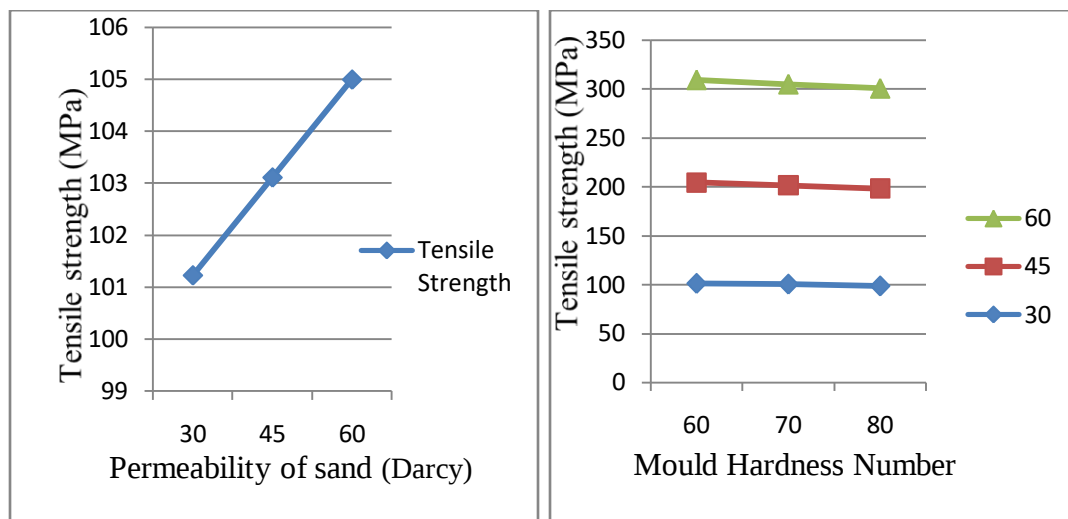
Figure 4.43: Effect of Permeability of sand and Mould Hardness Number on Tensile strength at Pouring Temperature of 750 °C
