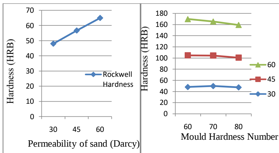
Figure 4.51: Effect of Permeability of sand on Hardness at pouring temperature of 750 0 C
