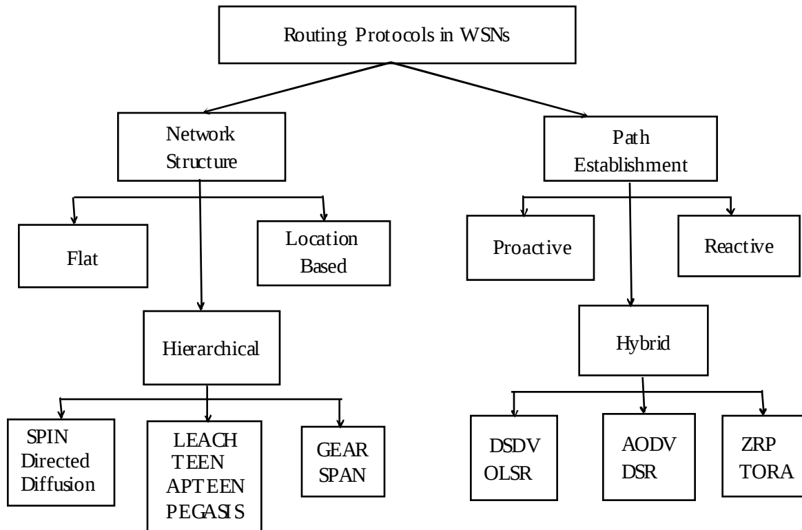
Figure 1: Routing Protocols in Wireless Sensor Networks
