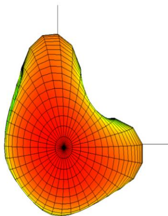
Fig 4. Radiation Pattern of Dual Polarization
