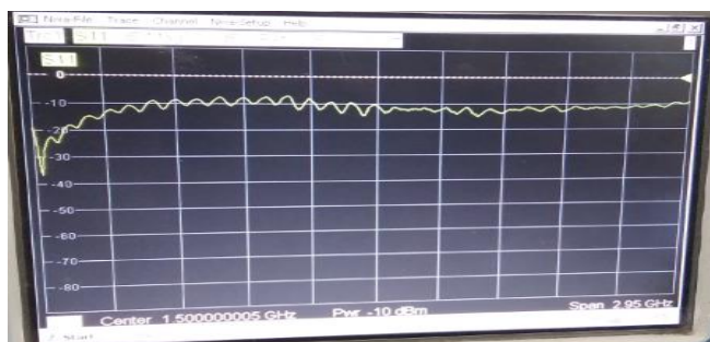
Fig 10. VNA Screenshot of S_{11}
