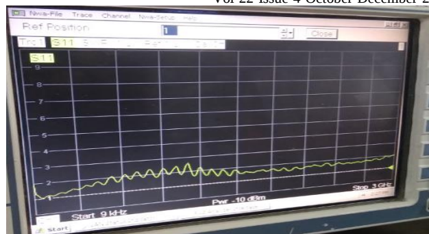
Fig 7. VNA Screenshot of VSWR at port one
