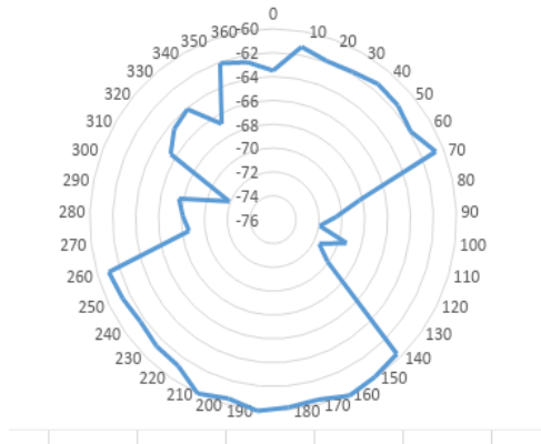
Fig.6. Monopole antenna's radiation pattern
